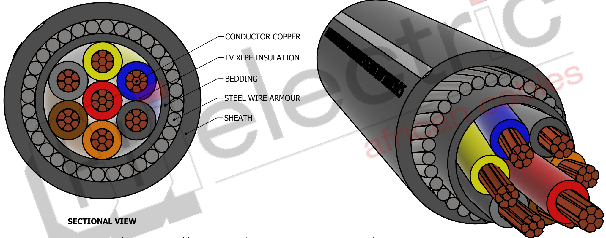
ISOMETRIC VIEW
