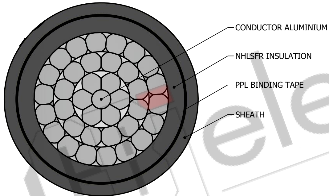
SECTIONAL VIEW
