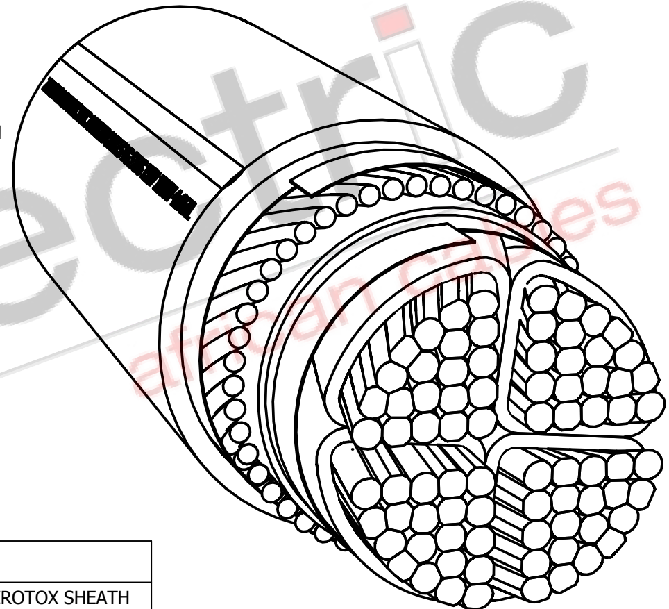
ISOMETRIC VIEW
