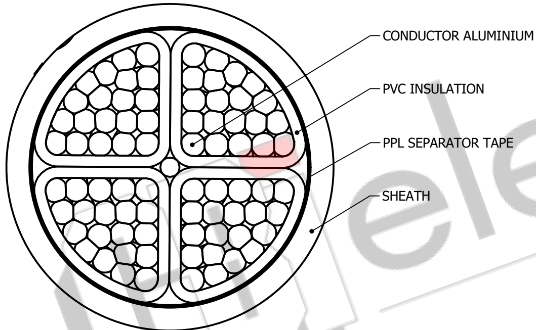
SECTIONAL VIEW
